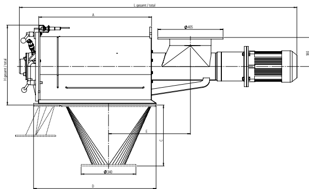
Ca. 1000 mm Siebkorbbaumaß Approx. 1000 mm sifter drum access space for maintenance
